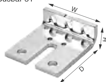
Busbar 5T
