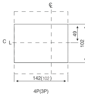
面板开孔尺寸 Panel cutout size
