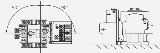
垂直或水平安装 Vertical mounting or level mounting
